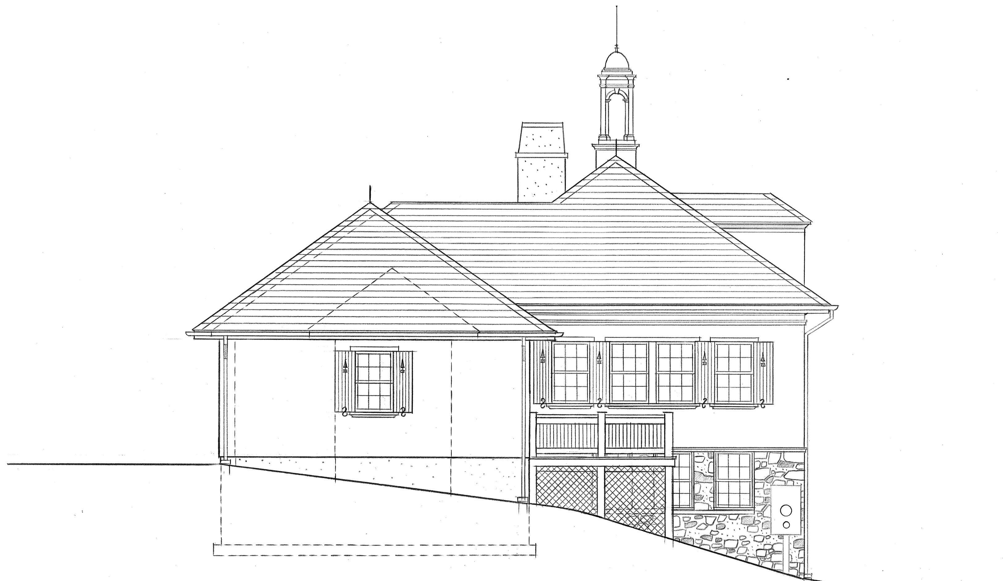
SOUTH ELEVATION
