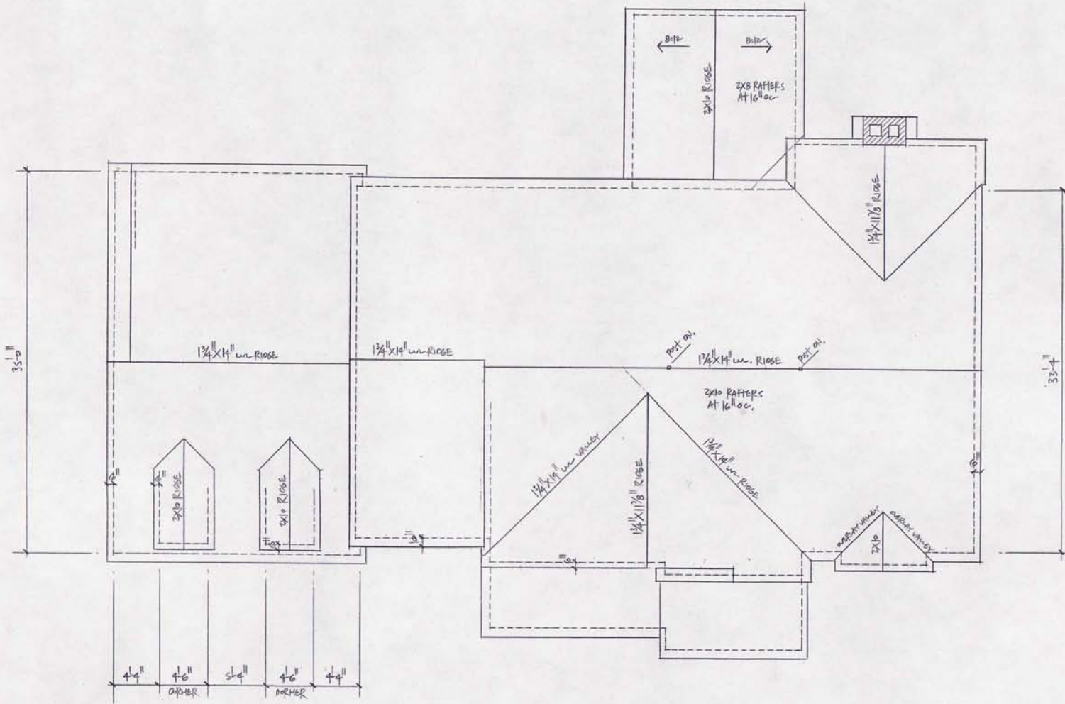
ROOF PLAN
