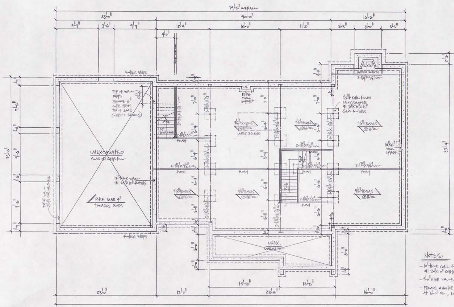
FOUNDATION PLAN 1/4" = 1'-0"
